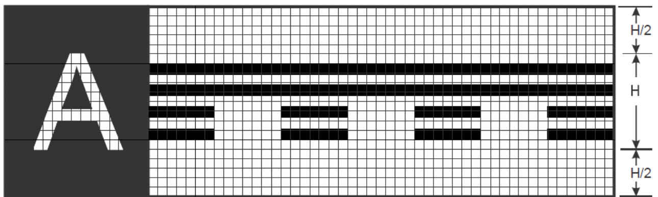
Runway vacated sign (with typical location sign)
