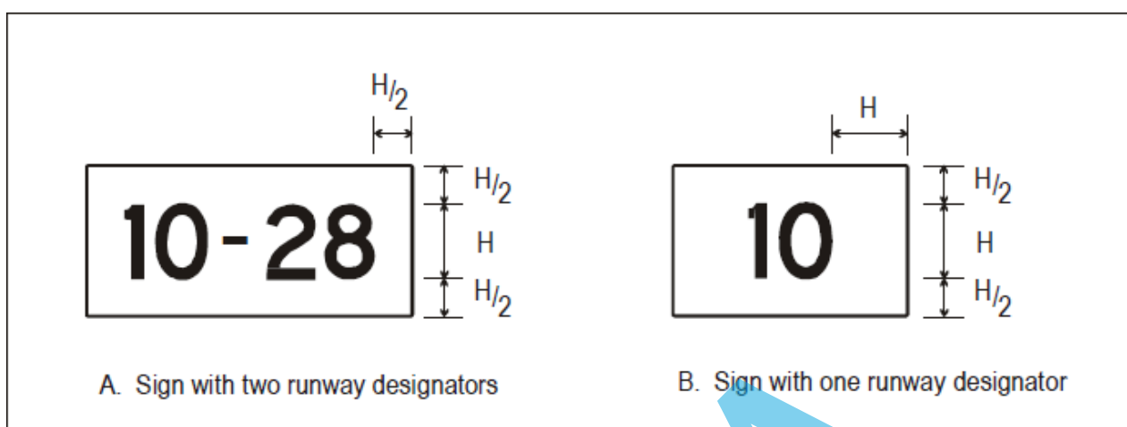
Figure A4-4. Sign dimensions
