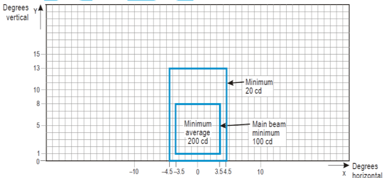
Figure A2-12. Isocandela diagram for taxiway centre line (15 m spacing), RELs, no-entry bar and stop bar lights in straight sections intended for use in runway visual range conditions of less than a value of 350 m where large offsets can occur and for low-intensity runway guard lights, Configuration B
