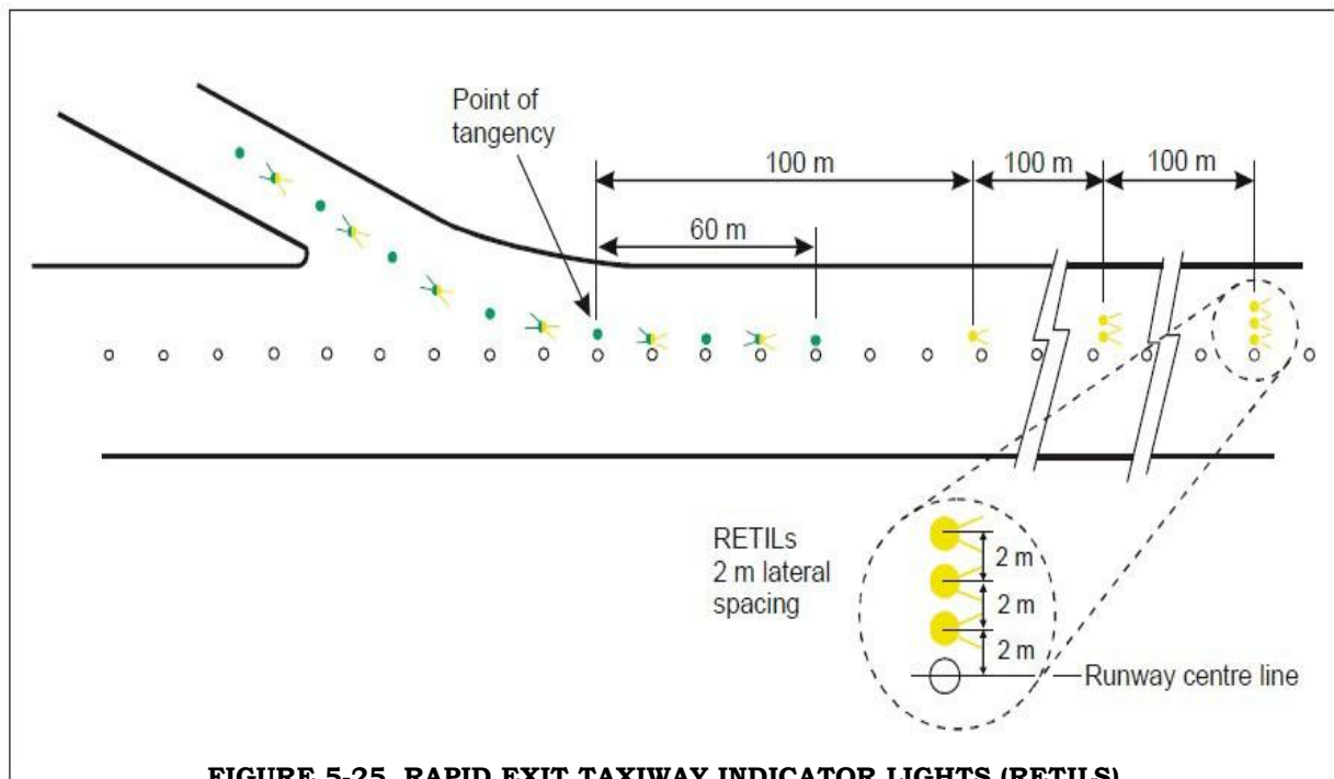
FIGURE 5-25. RAPID EXIT TAXIWAY INDICATOR LIGHTS (RETILS)
