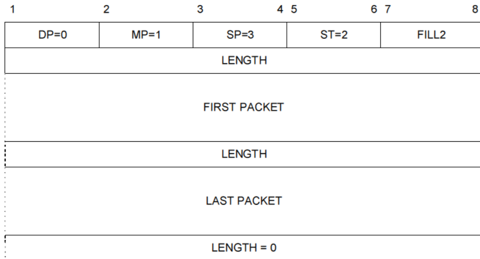
Figure 5-20. MULTIPLEX packet
