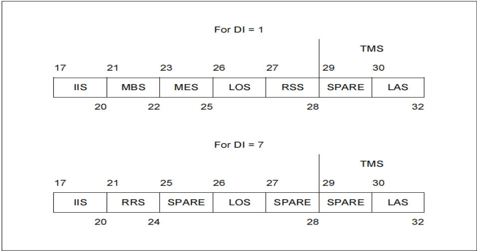
Figure 5-1. The SD field structure
