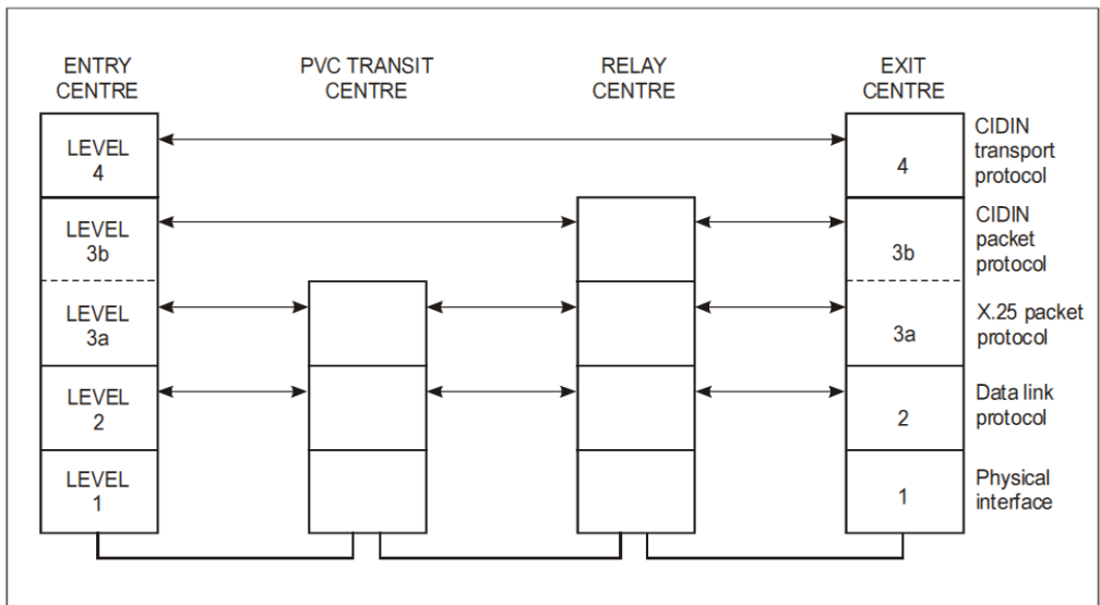
Figure 8-1. CIDIN protocol levels
