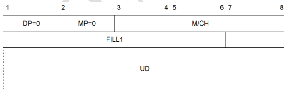
Figure 5-21. SHORT FORM MSP packet
