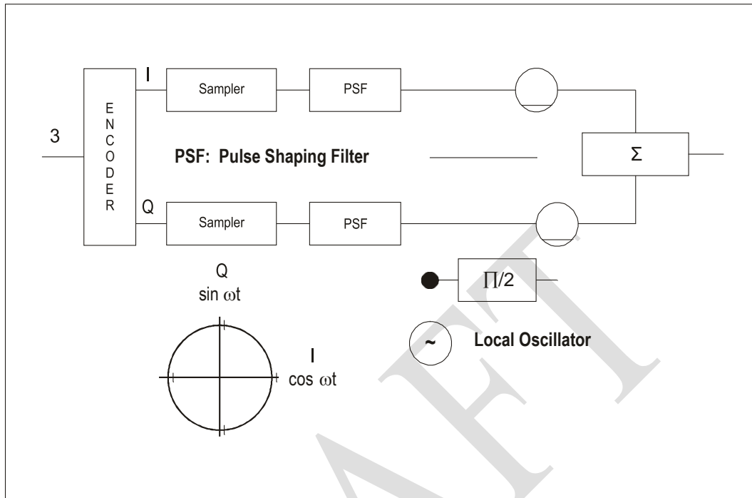
Figure B-19. Example data modulation
