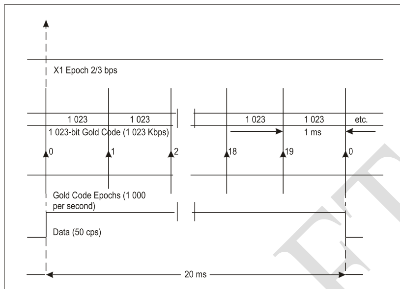
Figure B-1. C/A code timing relationships
