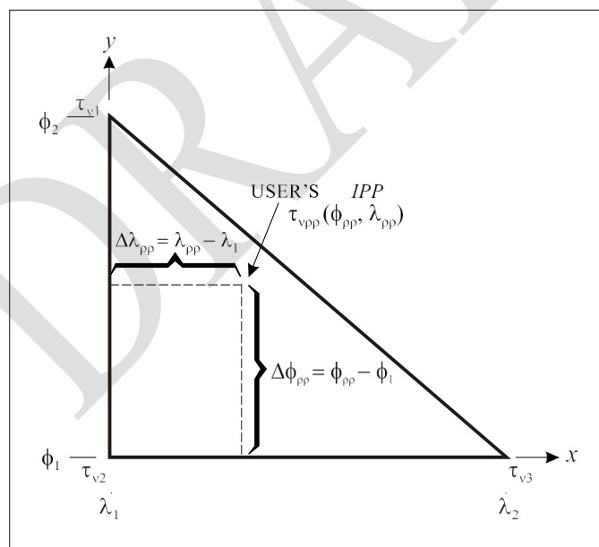
IGP numbering convention (three IGPs)
