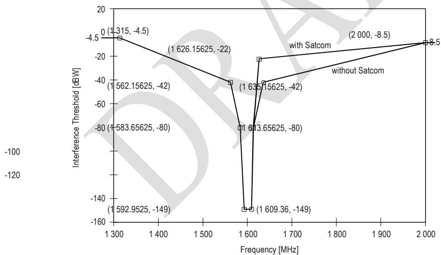
Figure B-16. CW interference thresholds for GLONASS receivers used for precision approach
