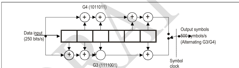
Figure B-11. Convolutional encoding
