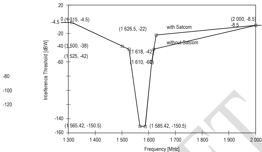
Figure B-15. CW interference thresholds for GPS and SBAS receivers used for precision approach
