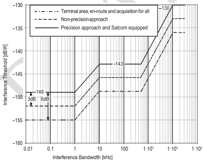
Interference thresholds versus bandwidth for
