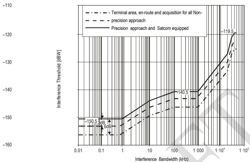
Figure B-17. Interference thresholds versus bandwidth for GPS and SBAS receivers
