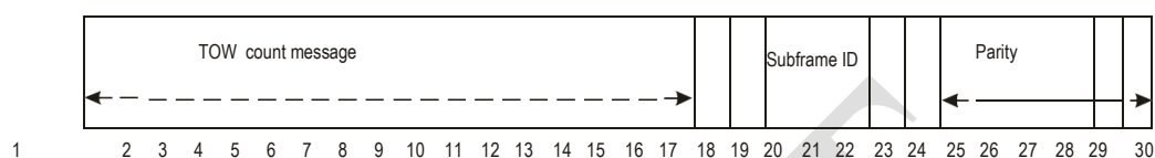
Figure B-4. HOW format
