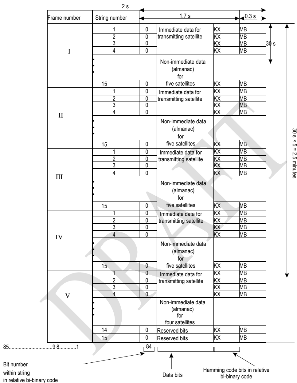
Figure B-7. Superframe structure
