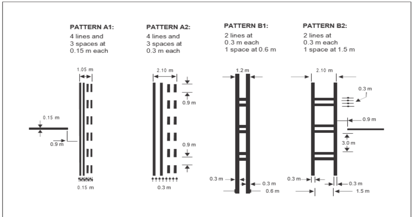
Figure 5-8. Runway-holding position markings
