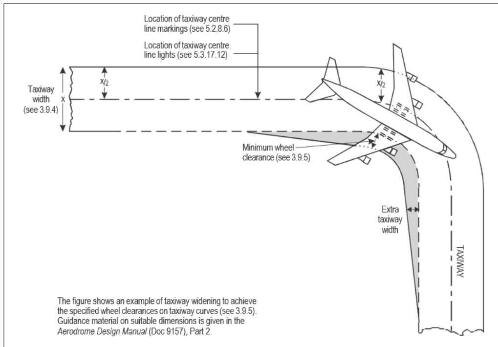
Figure 3-2. Taxiway curve
