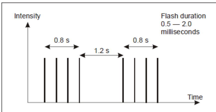
Figure 5-10. Heliport beacon flash characteristics
