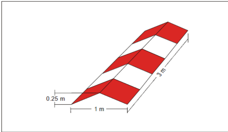
Figure 5-5. Runway-type FATO edge marker
