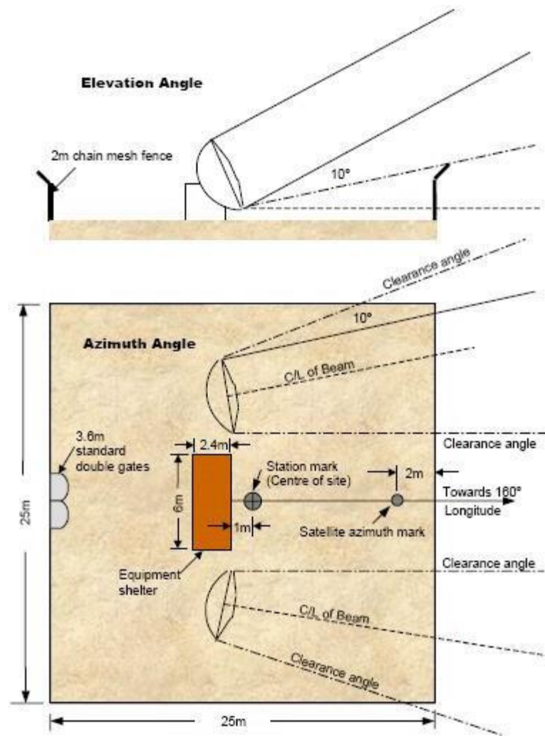
Figure 12: COMMUNICATIONS SATELLITE GROUND STATION MANNED CENTRE SITE
