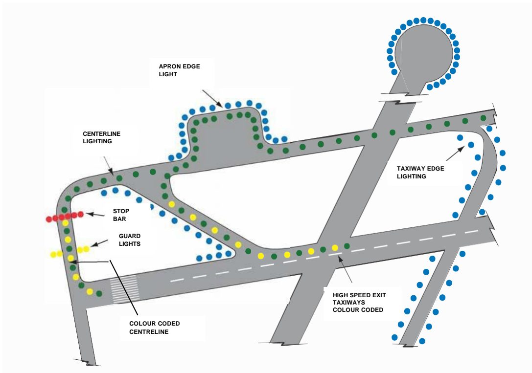
Figure 1.7 Taxiway Lighting
