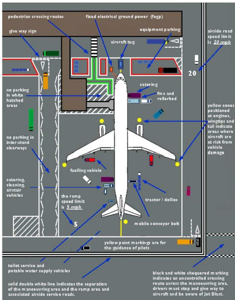
Figure 2.3 Typical Stand Layout and Markings
