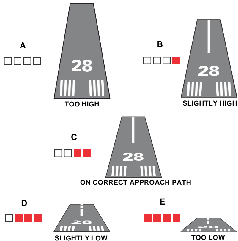
Figure 1.4 A Typical PAPI System
