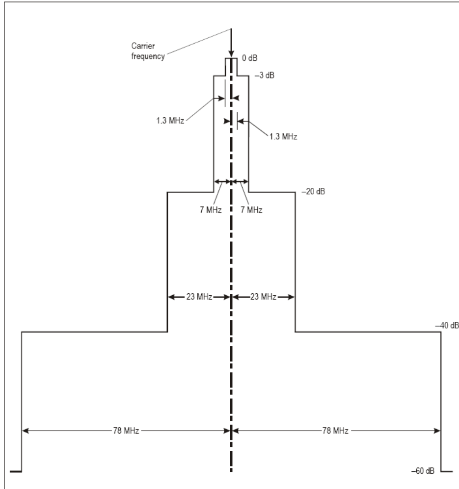
Figure 3-2. Required spectrum limits for interrogator transmitter
