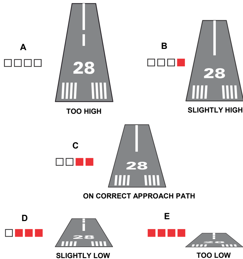
Figure 1.4 A Typical PAPI System
