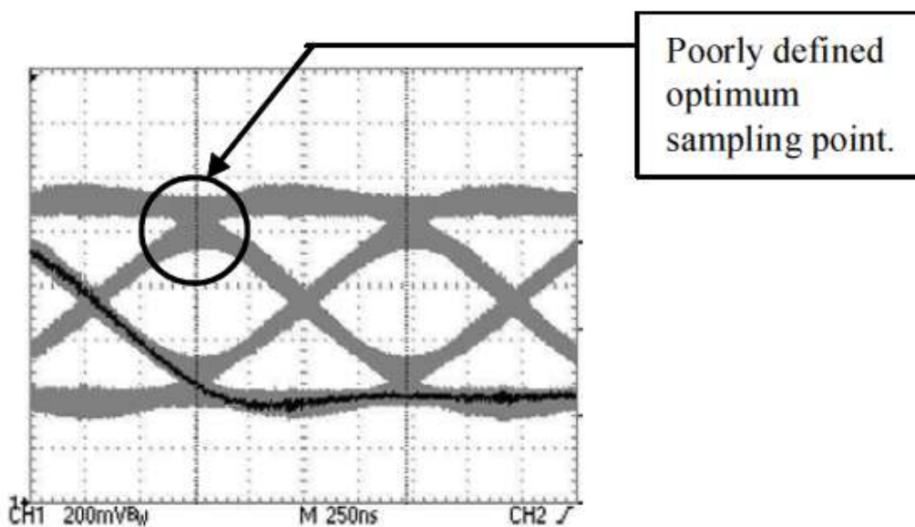
Figure 12-4. Distorted eye diagram
