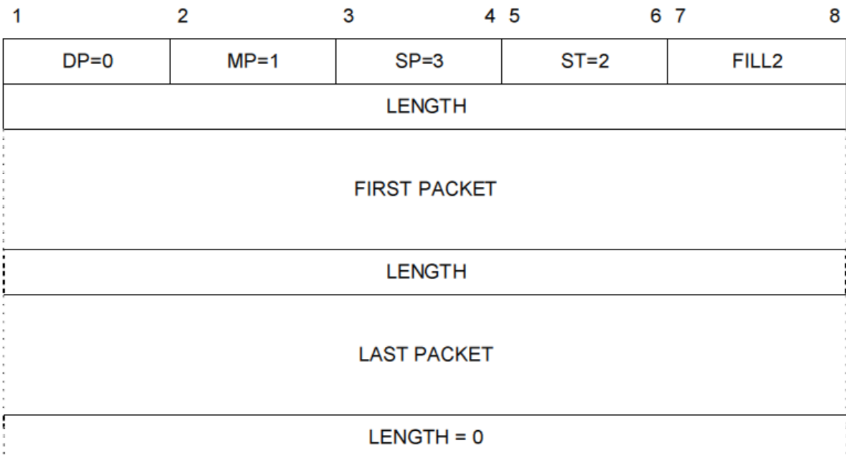
Figure 5-20. MULTIPLEX packet
