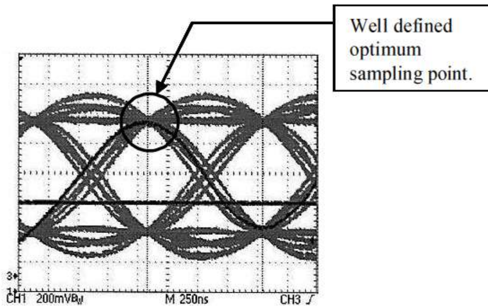
Figure 12-3. Ideal eye diagram
