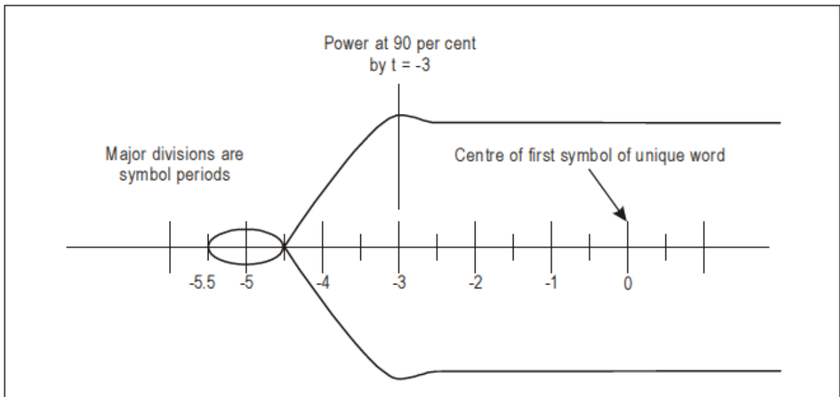
Figure 6-1. Transmitter power stabilization
