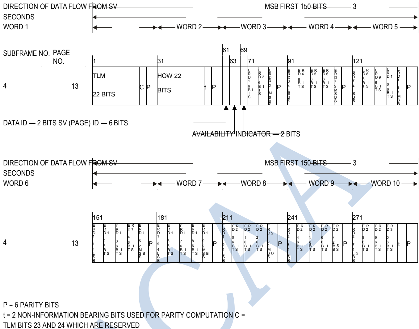
Figure B-6. Data format (10 of 11)
