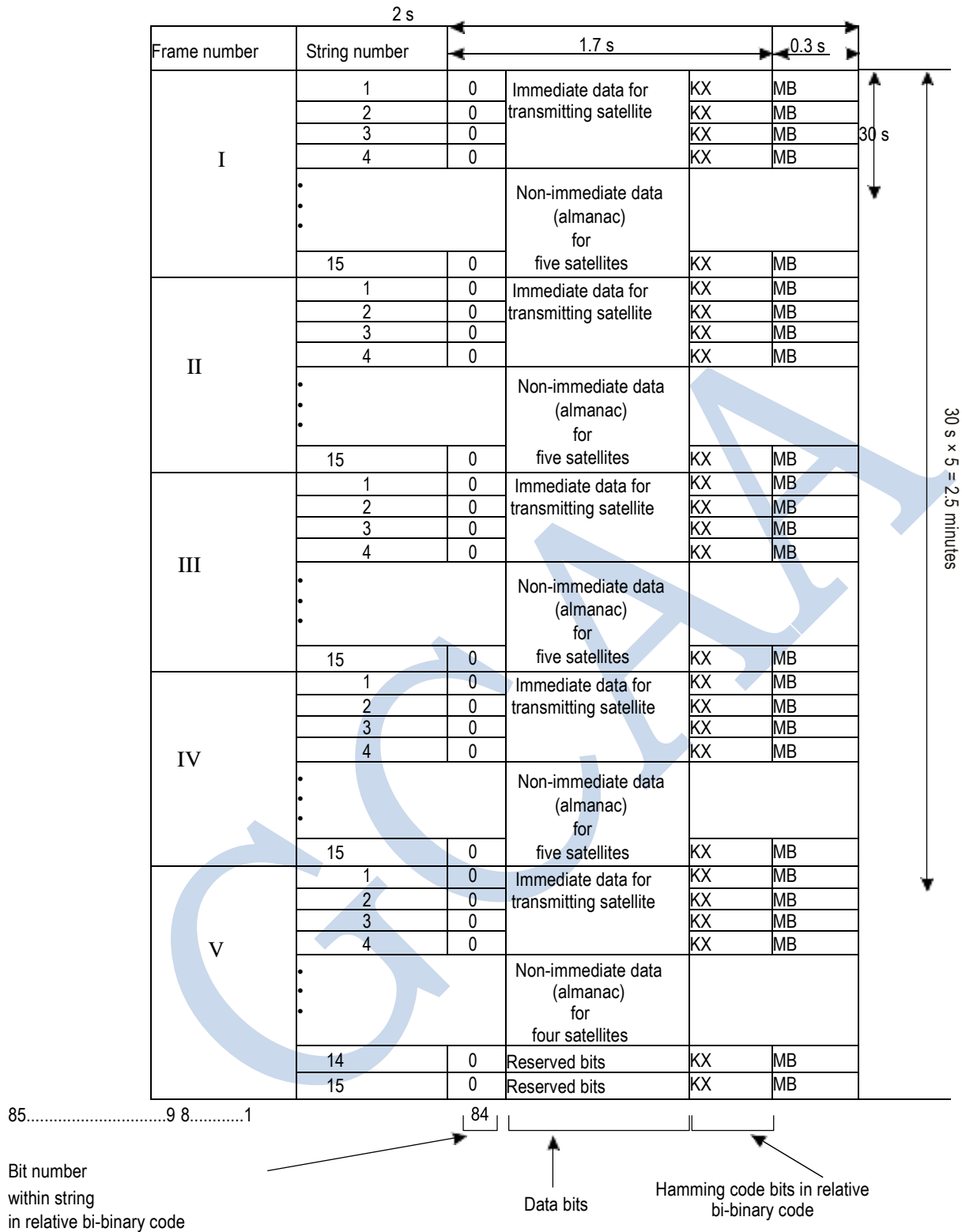
Figure B-7. Superframe structure
