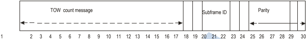
Figure B-4. HOW format
