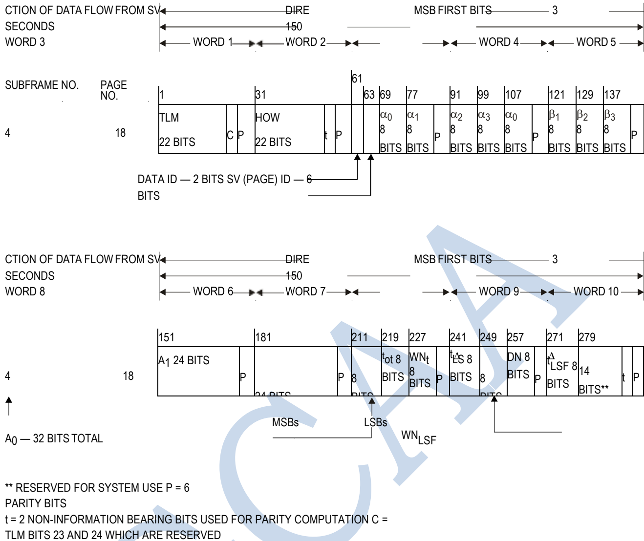
Figure B-6. Data format (8 of 11)
