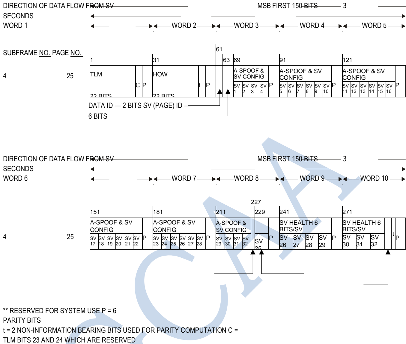
Figure B-6. Data format (9 of 11)
