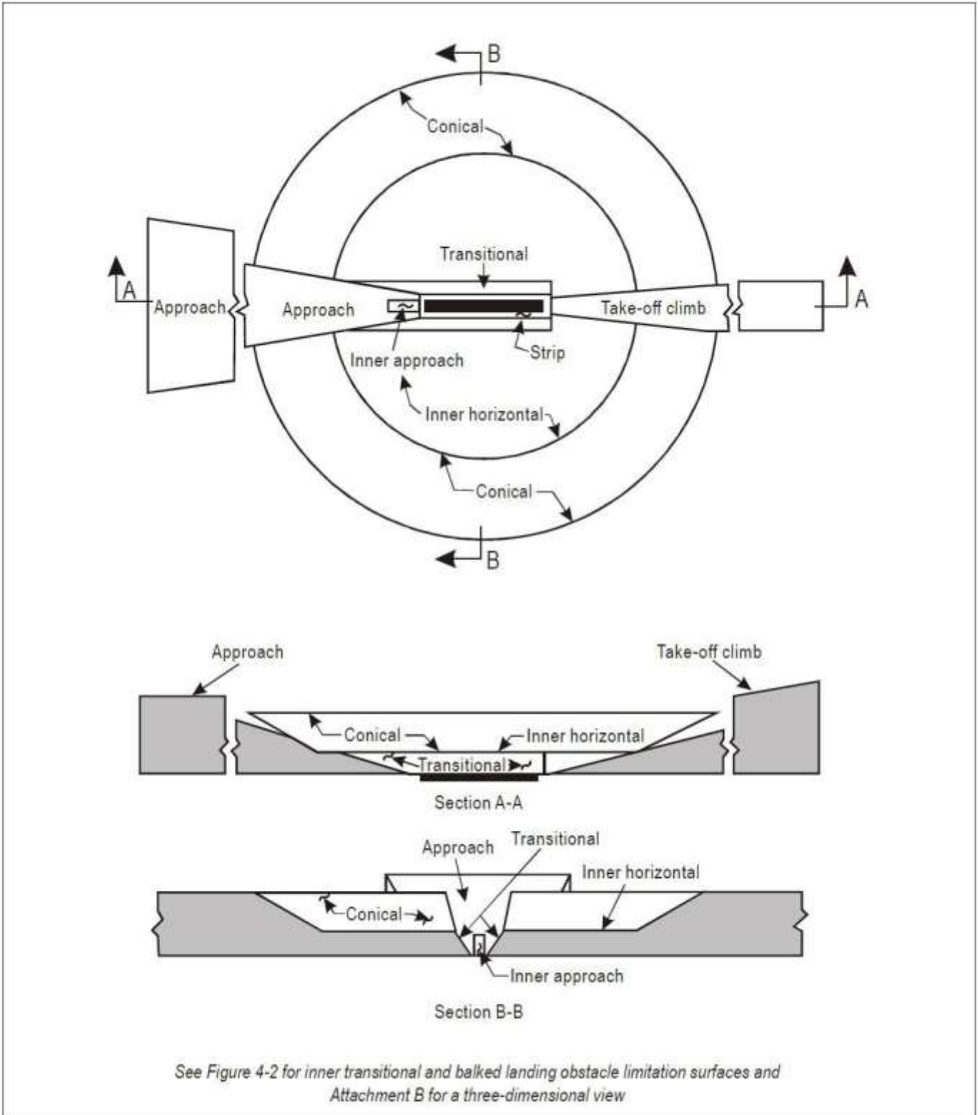
Figure 4-1. Obstacle limitation surfaces
