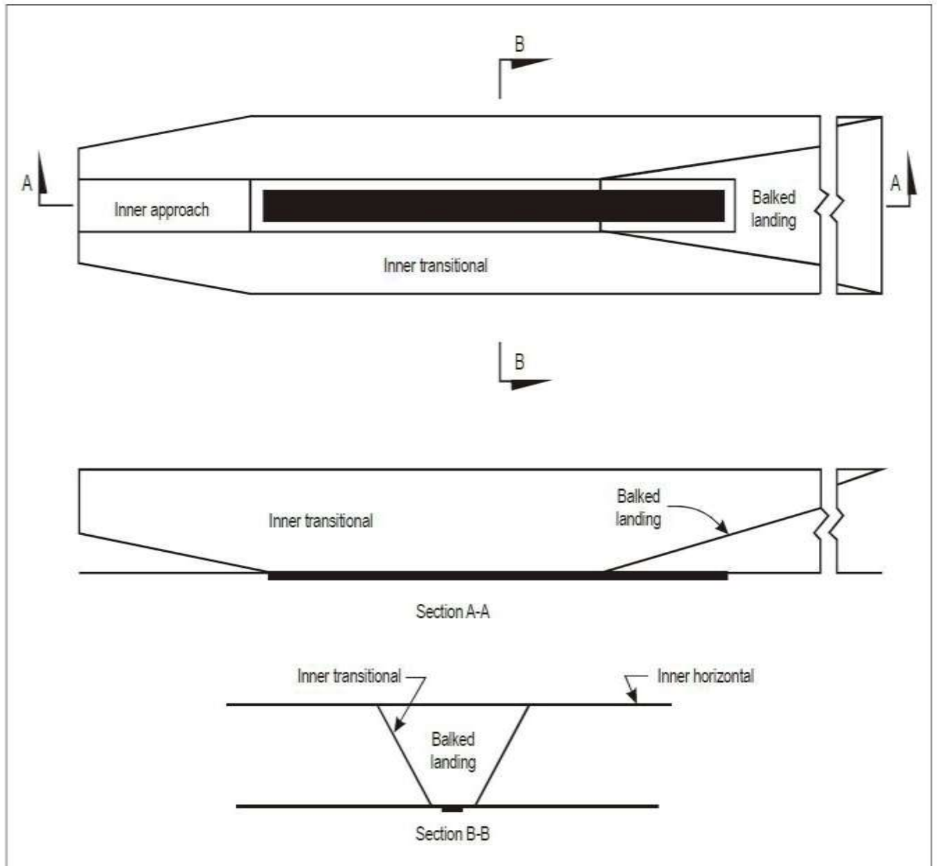
Figure 4-2. Inner approach, inner transitional and bailed landing obstacle limitation surfaces
