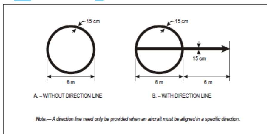
Figure 5-9. VOR aerodrome checkpoint marking
