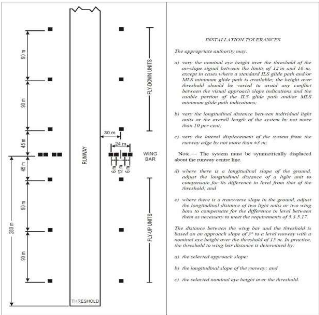
Figure 5-17. Siting of light units for T-VASIS
