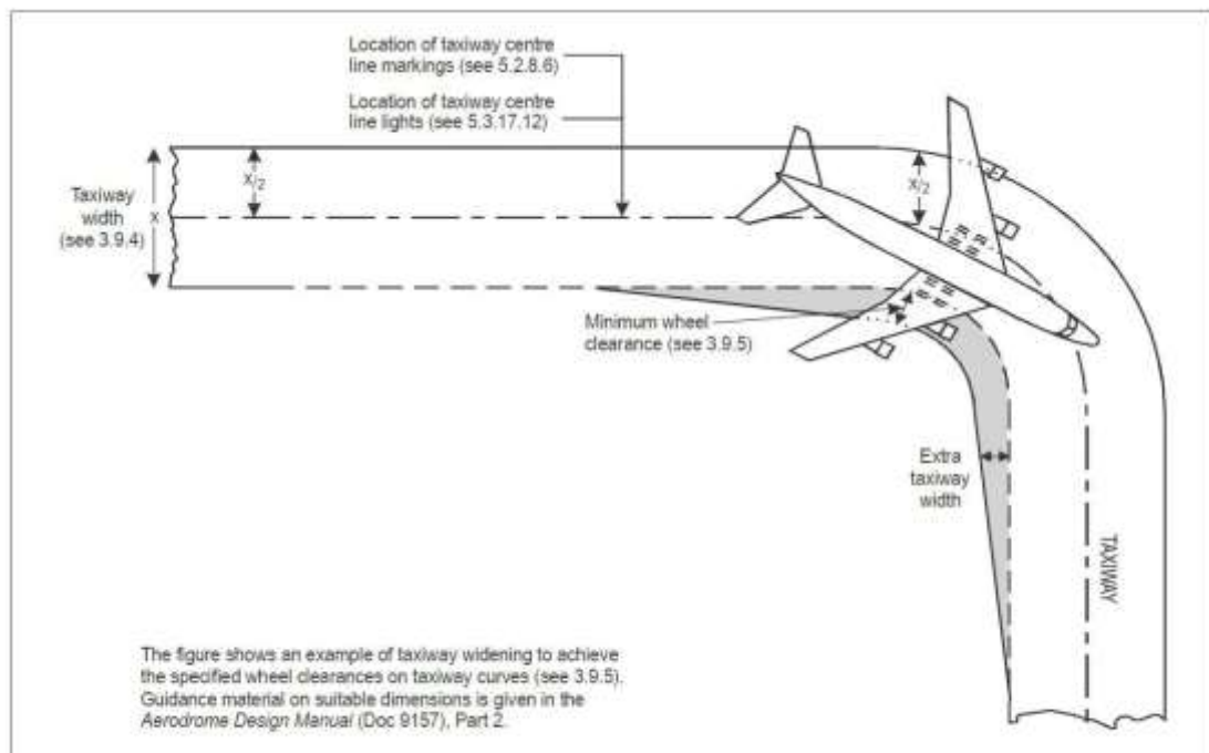
Figure 3-2. Taxiway curve
