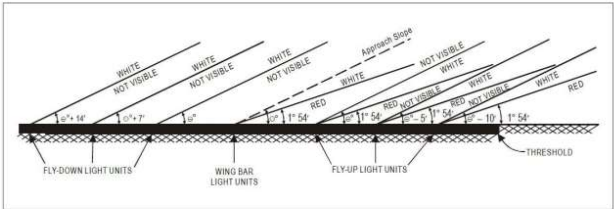
Figure 5-18. Light beams and elevation settings of T-VASIS and AT-VASIS
