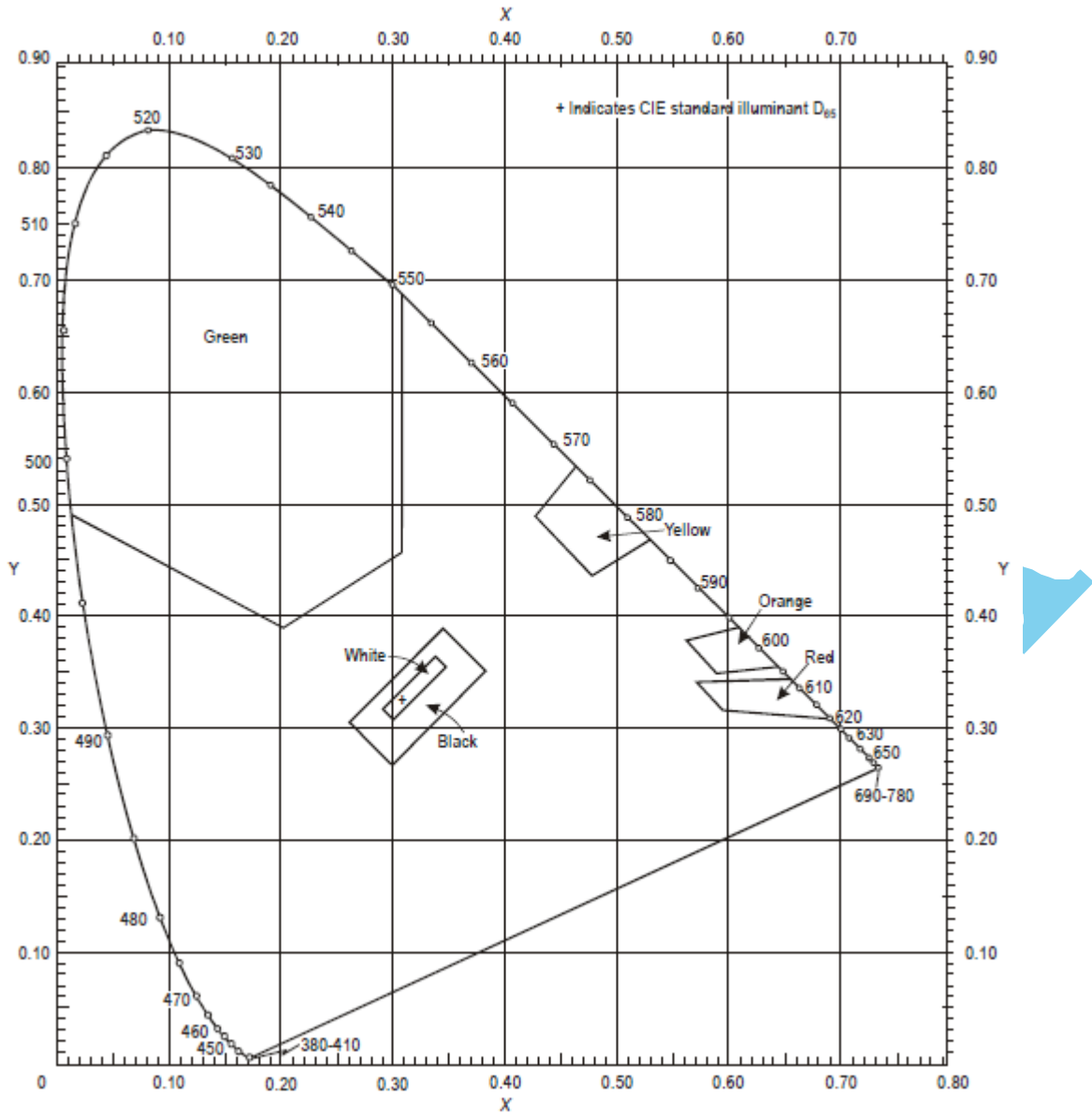
Figure A1-2. Ordinary colours for markings and externally illuminated signs and panels
