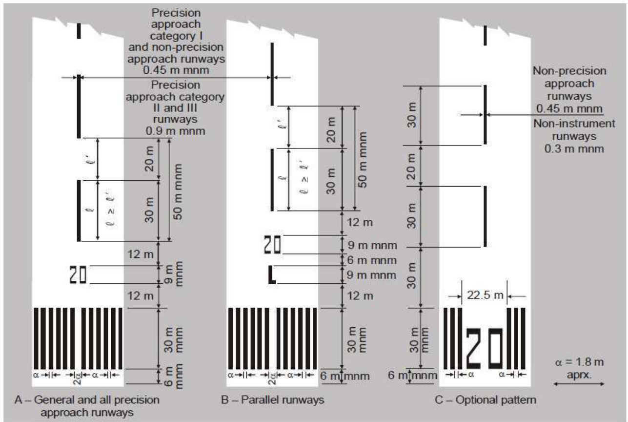
Figure 5-2. Runway designation, centre line and threshold markings
