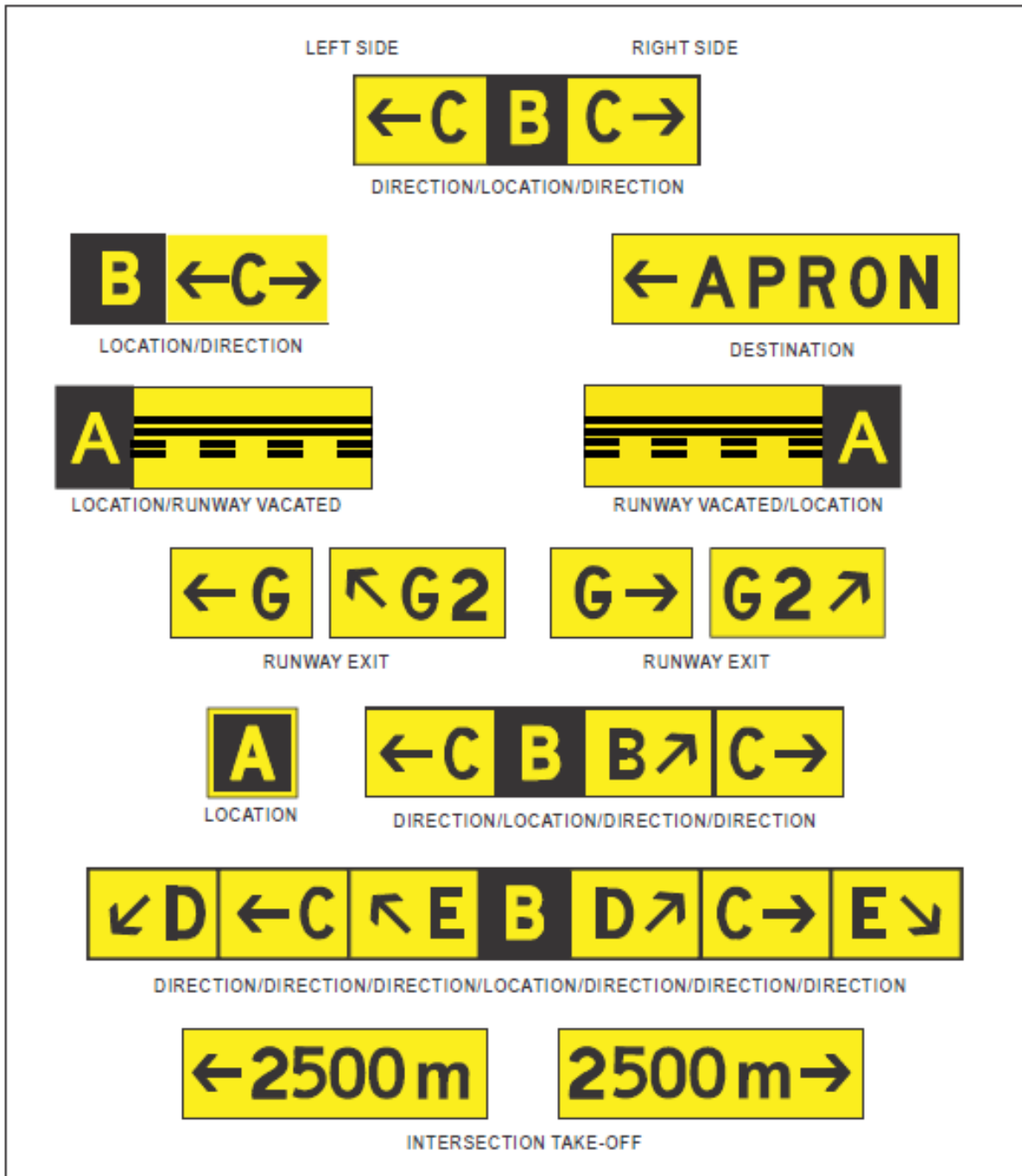
Figure 5-31. Information signs
