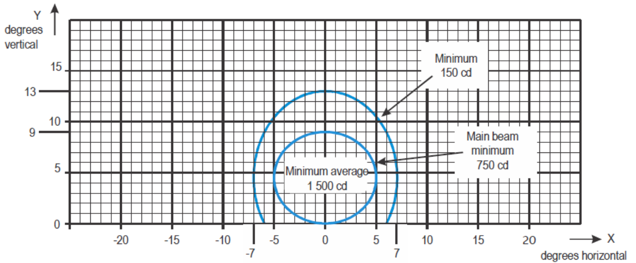
Figure A2-25. Isocandela diagram for each light in high-intensity runway guard lights, Configuration A
