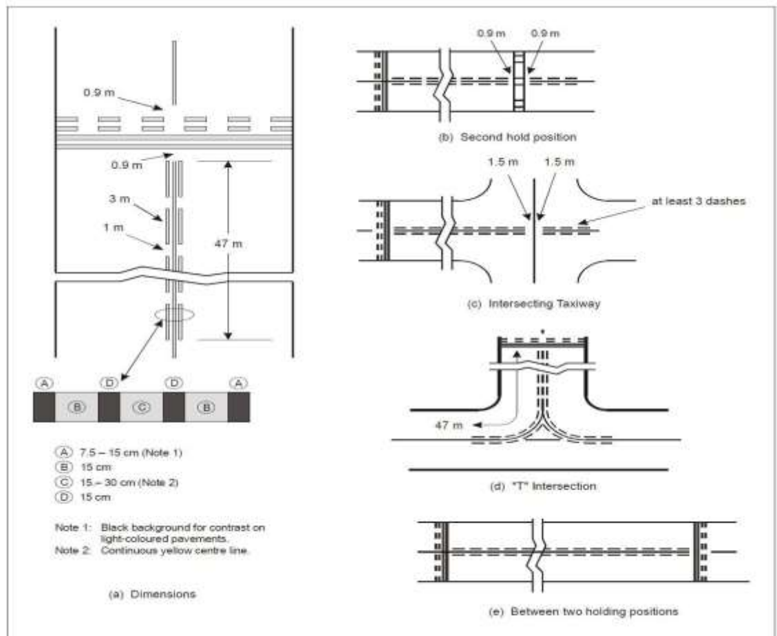
Figure 5-7. Enhanced taxiway centre line marking
