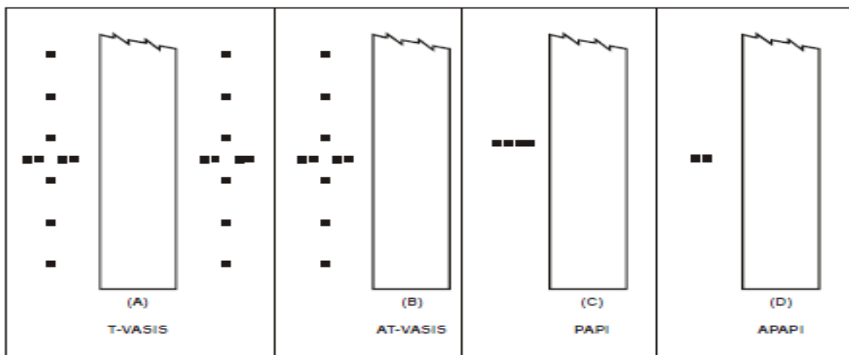
FIGURE 5-16. VISUAL APPROACH SLOPE INDICATOR SYSTEMS
