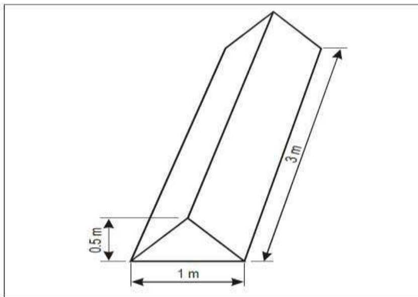
Figure 5-34. Boundary markers
