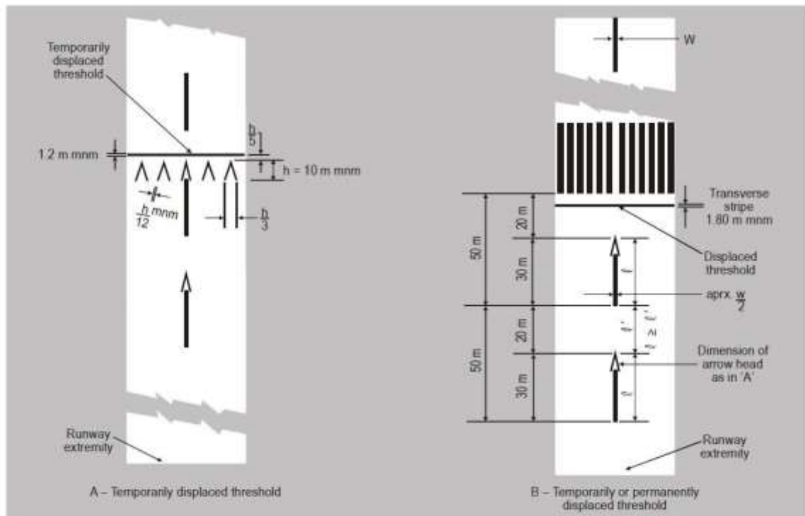
Figure 5-4. Displaced threshold markings
