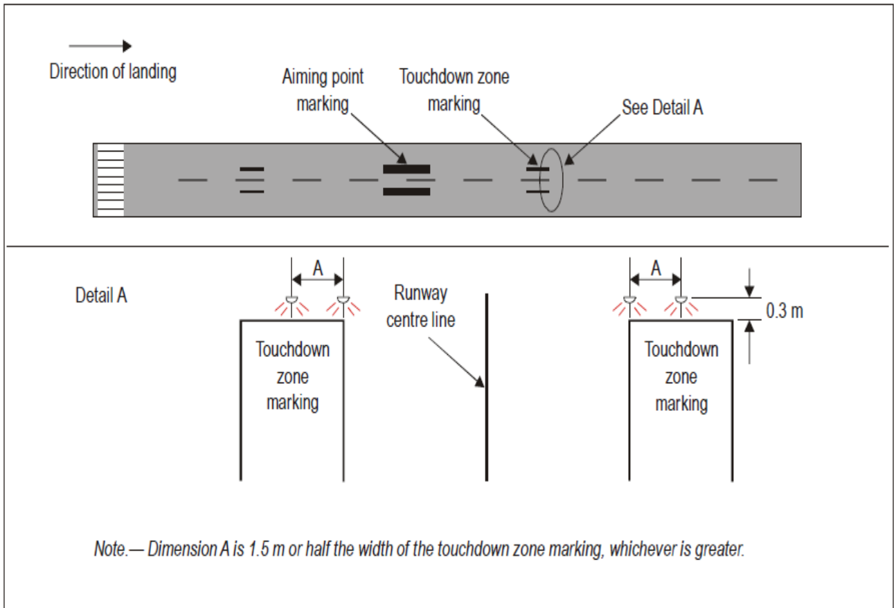
FIGURE 5-24. SIMPLE TOUCHDOWN ZONE LIGHTING
