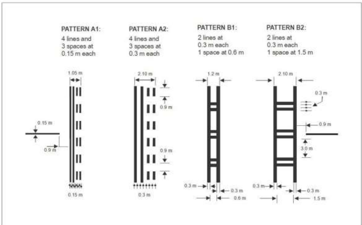
Figure 5-8. Runway-holding position markings Note. — Patterns A1 and B1 are no longer valid after 2026.
