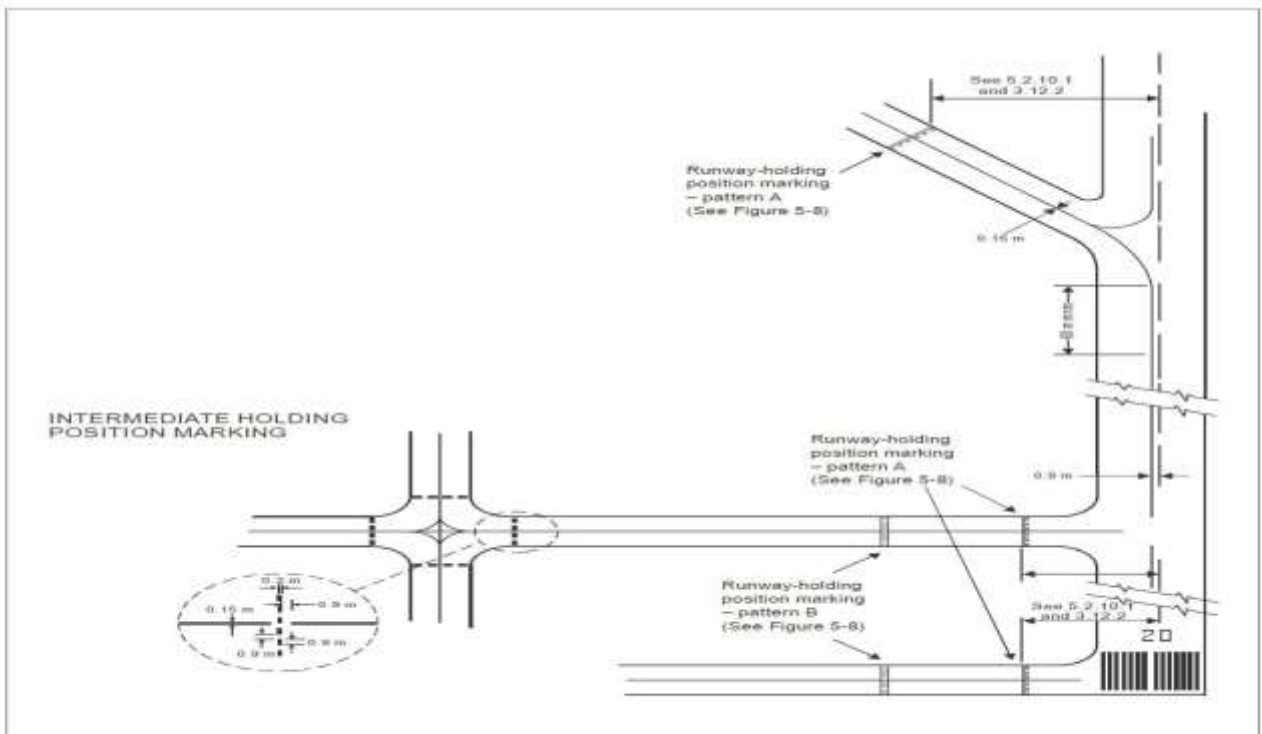
Figure 5-6. Taxiway markings (shown with basic runway markings)
