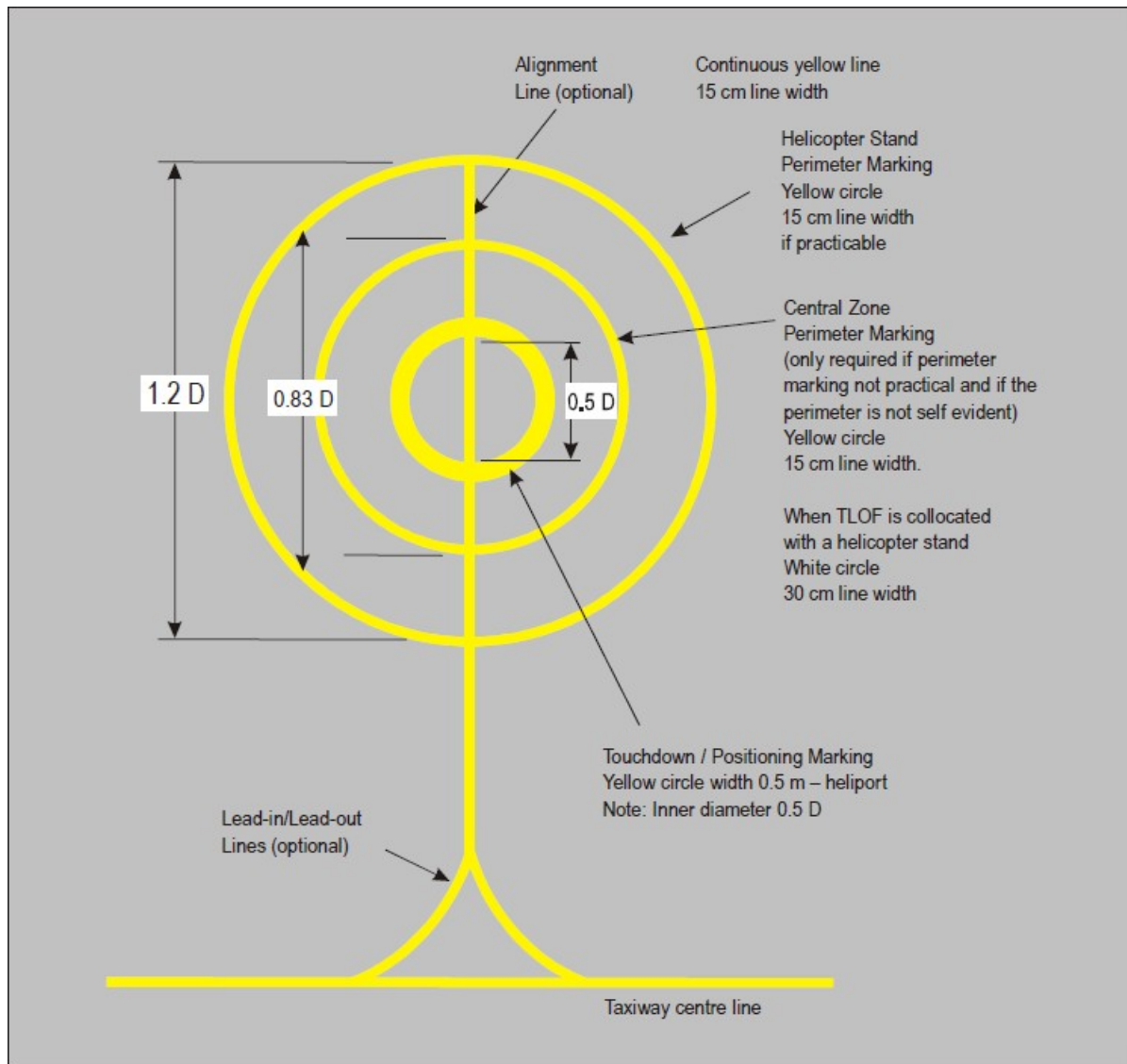
Figure 5-8. Helicopter stand markings
