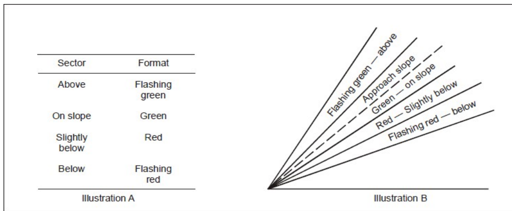
Figure 5-15. HAPI signal format
