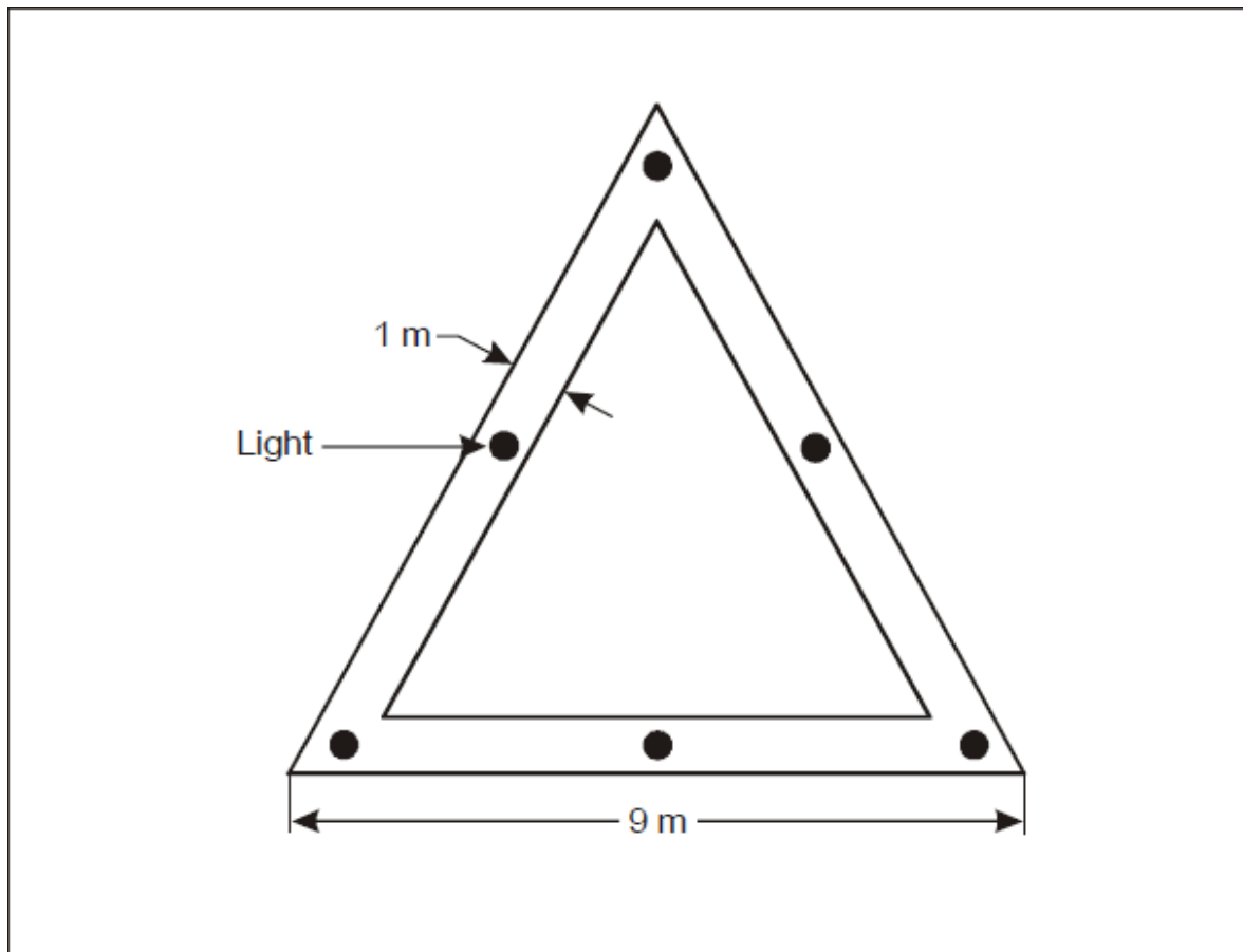
Figure 5-6. Aiming point marking
