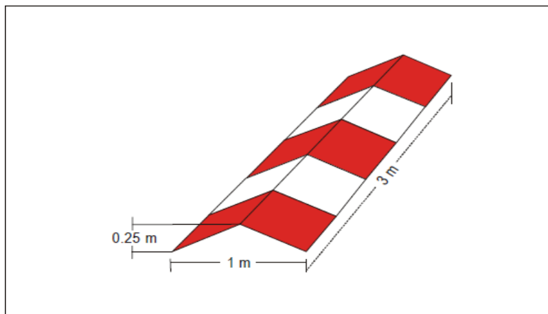
Figure 5-5. Runway-type FATO edge marker
