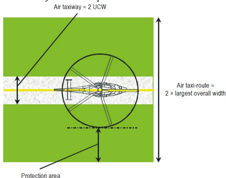
Figure 3-3. Helicopter air taxi-route/taxiway
