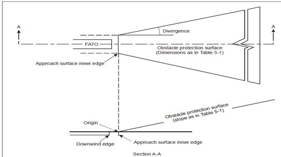
Figure 5-14. Obstacle protection surface for visual approach slope indicator systems
