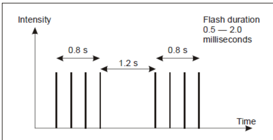
Figure 5-10. Heliport beacon flash characteristics
