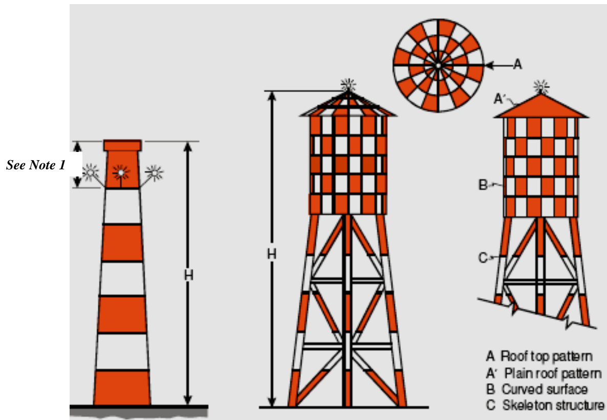
Figure 1(b) – Marking and lighting of tall structures
